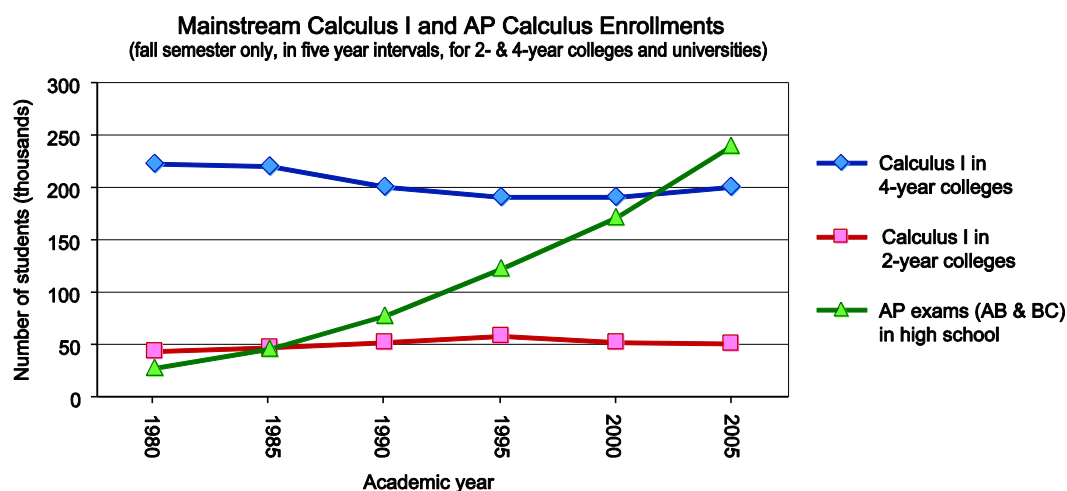
Figure 1. Comparison of the number of students taking the Advanced Placement (AP) calculus exams with the number taking first-semester mainstream calculus during the fall term at five-year intervals, 1980-2005. (Source: “The Crisis of Calculus,” David M. Bressoud. In Launchings from the CUPM Curriculum Guide , April, 2007. 1
